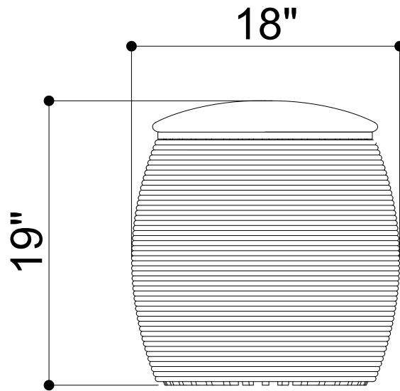
2 FRONT VIEW
